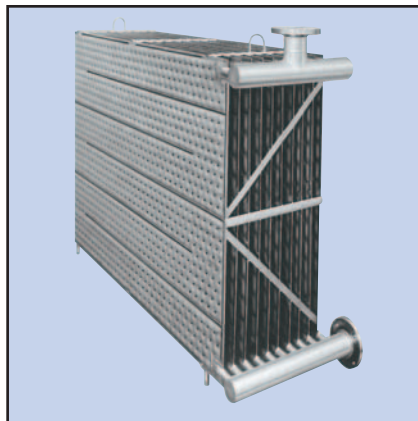
Bank for Cooling
