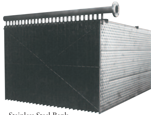
Stainless Steel Bank for Heat Recovery
